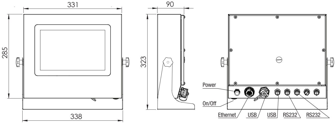
PX10 Housing
