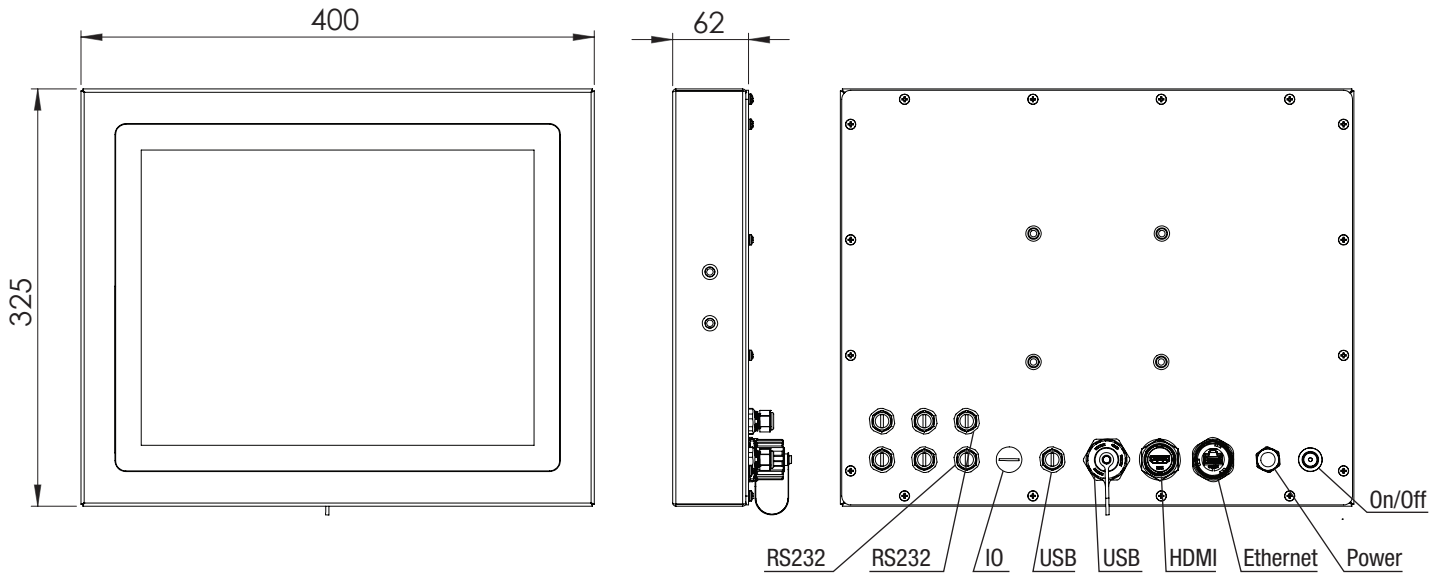
PX15 Housing
